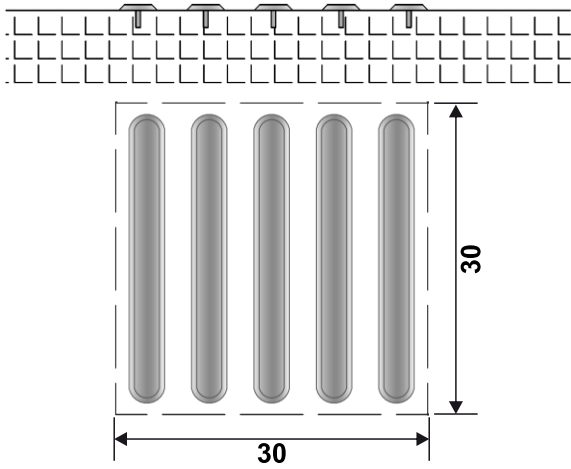
28 cm stainless steel hidden screw tangible surface walk line.
