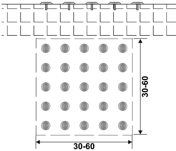
28 mm stainless steel hidden screw tangible surface waiting points.
