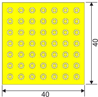
40*40 cm polyurethane tangible surface waiting plate.
