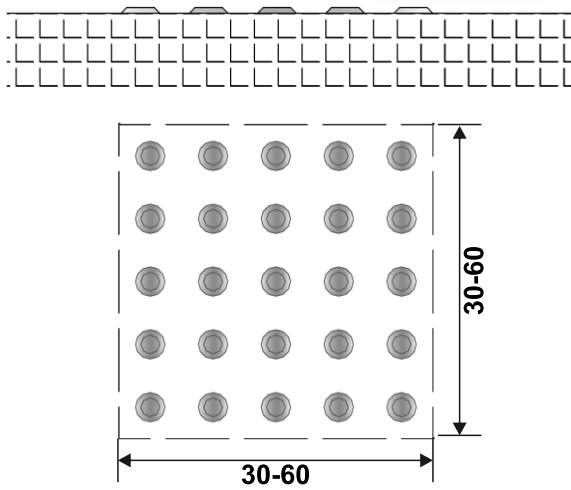
28 mm stainless steel self-adhesive tangible surface waiting points.
