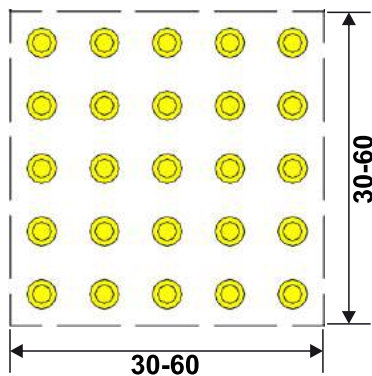
28 mm polyurethane hidden screw tangible surface waiting points.
