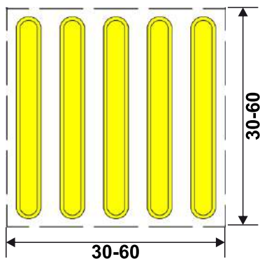
28 cm polyurethane hidden screw tangible surface walk line.
