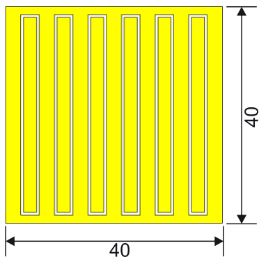
40*40 cm polyurethane tangible surface walk plate.
