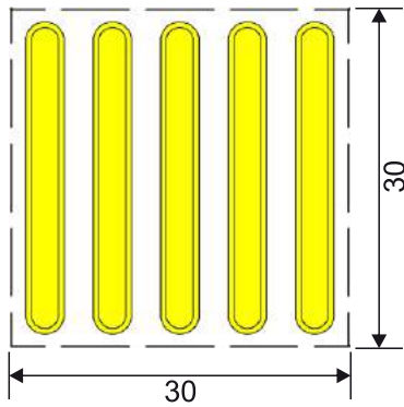
28 cm polyurethane self-adhesive tangible surface walk line.
