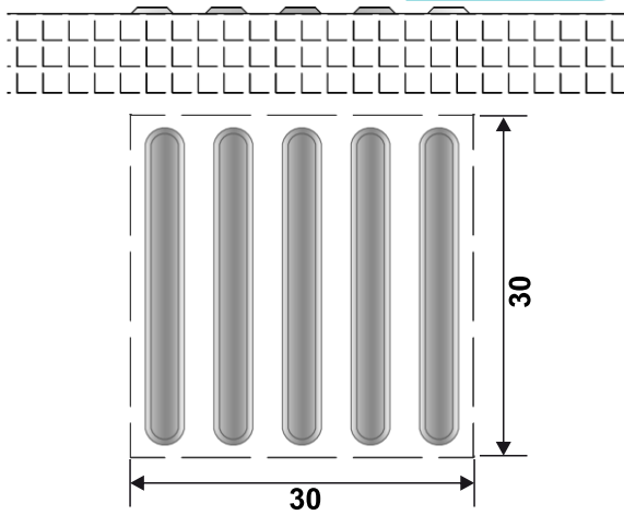
28 cm stainless steel self-adhesive tangible surface walk line.
